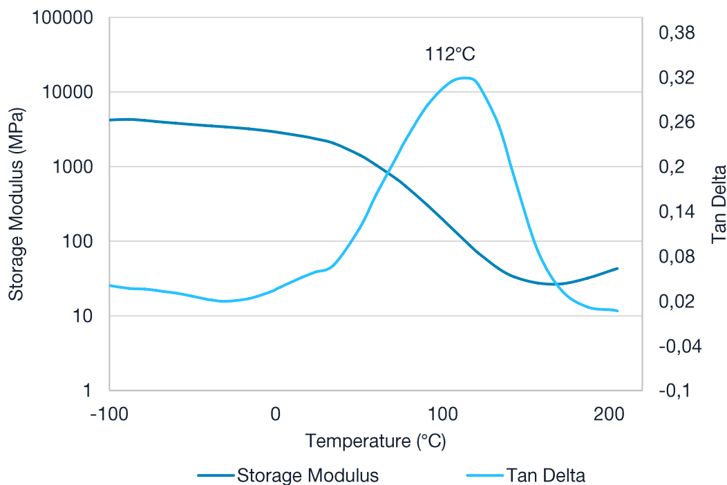
DMA curve
