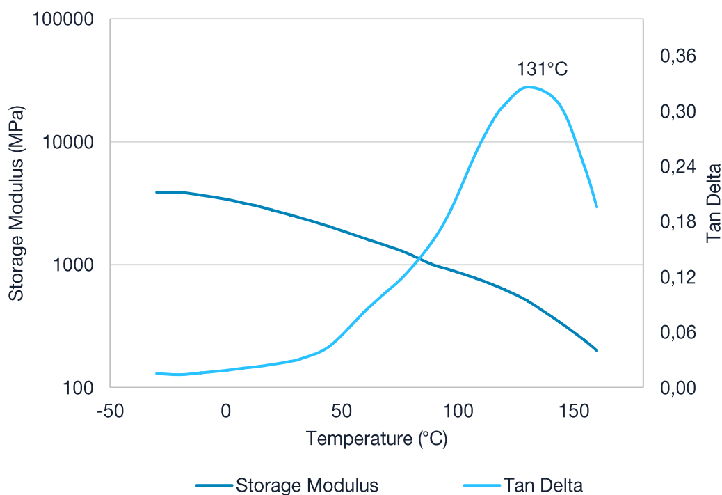
DMA curve
